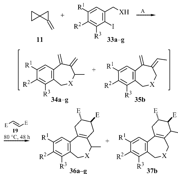
Scheme 5. One-pot, two-step, three-component queuing cascade involving methylenespiropentane ( 11 ), o -iodobenzyl alcohols and -amines 33a–g as well as dimethyl fumarate ( 19 ). (A) Pd(OAc) 2 , TFP, Et 3 N, DMF, 80 °C, 3 h. E = CO 2 Me. For details see Table 1.
