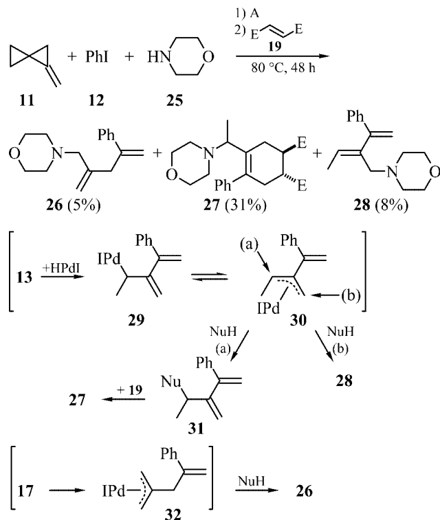
Scheme 4. One-pot palladium-catalyzed reaction of methylenespiropentane ( 11 ) with iodobenzene ( 12 ) and morpholine ( 25 ) with subsequent trapping of a formed 1,3-diene by dimethyl fumarate ( 19 ). (A) Pd(OAc) 2 , TFP, Et 3 N, DMF, 80 °C, 3 h. NuH = morpholine. E = CO 2 Me.
