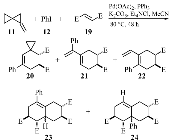
Scheme 3. A domino Heck–Diels–Alder reaction involving methylenespiropentane ( 11 ), iodobenzene ( 12 ) and dimethyl fumarate ( 19 ). E = CO 2 Me.
