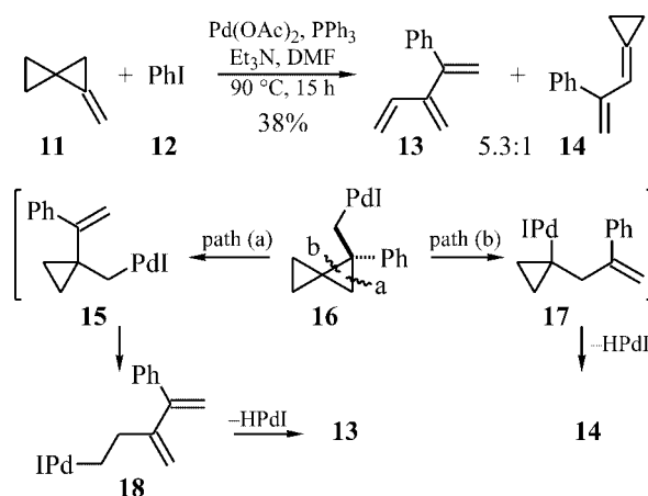
Scheme 2. Heck coupling of methylenespiropentane ( 11 ) with iodobenzene ( 12 ).
