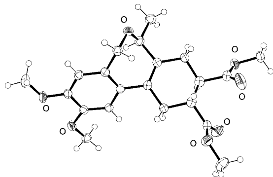
Figure 1. Structure of compound 36c (major diastereomer) in the crystal. [8] C_{21}H_{26}O_7 (390.42); crystal size 0.30 \times 0.30 \times 0.30 mm; triclinic; a = 727.68(7) , b = 1188.90(12) , c = 1290.95(12) pm; \alpha = 109.904(7)^\circ , \beta = 93.316(8)^\circ , \gamma = 106.331(8)^\circ ; V = 0.99306(17) nm 3 ; Z = 2 ; space group P1 ; T = 133(2) K; \rho = 1.306 Mg/m 3 ; \mu = 0.098 mm -1 ; F_o = 416 ; \theta range for data collection: 1.70 – 24.79^\circ ; reflections collected: 11159; R_{int} = 3356 [0.0370]; data/restraints/parameters: 3356/0/253; Goof on F^2 = 1.115 ; final R indices [ I > 2\sigma(I) ]: R_1 = 0.0505 , wR_2 = 0.1480 ; R indices (all data): R_1 = 0.0672 , wR_2 = 0.1562 ; largest difference peak/hole: 0.839/-0.314 e Å -3 .
