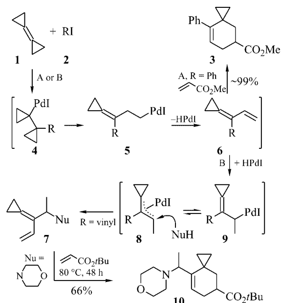
Scheme 1. Two recently developed one-pot reactions of bicyclopopylidene ( 1 ) involving palladium-catalyzed Heck couplings, cyclopropylcarbinyl to homoallyl rearrangements, \beta -dehydropalladations, rehydropalladation and Diels–Alder reactions. (A) \text{Pd}(\text{OAc})_2 , \text{PPh}_3 , \text{Et}_4\text{NCl} , \text{K}_2\text{CO}_3 , \text{Me}_3\text{CN} , 80 °C, 48 h. (B) \text{Pd}(\text{OAc})_2 , TFP, \text{Et}_3\text{N} , DMF, 80 °C, 2 h.
